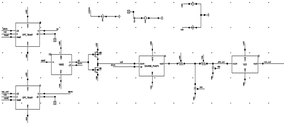
Figure2. Schematic of Phase locked loop
