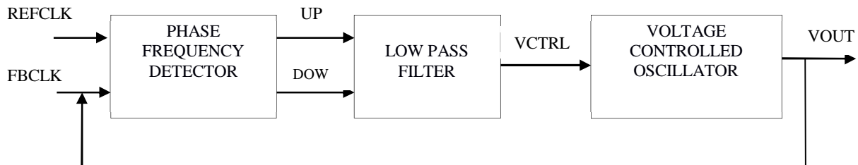
Figure1. Functional block diagram of Phase locked loop
