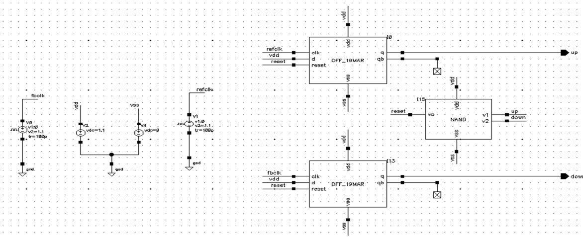
Figure3. Phase frequency detector
