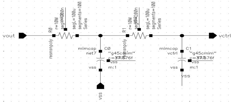
Figure6. Low pass filter
