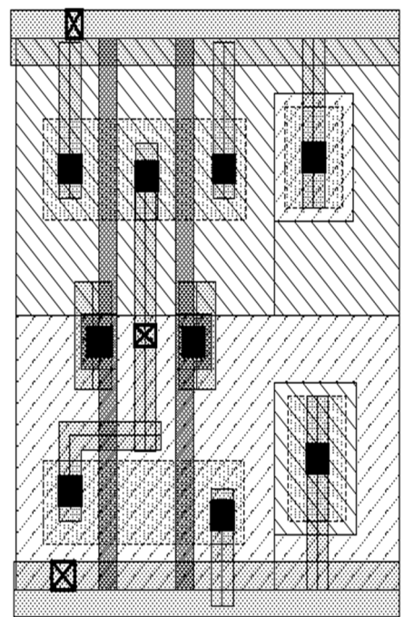
Figure5. Standard cell layout of NAND gate
